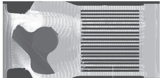
Cavitation breaker
