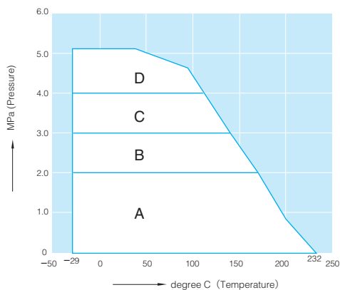
334A-class 300 Actuator Division (Body Material : WCB)
