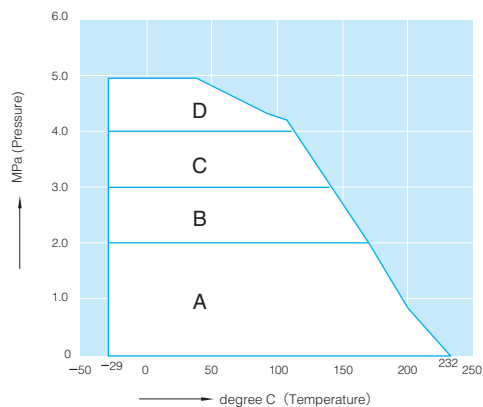
334A-class 300 Actuator Division (Body Material : CF8M)
