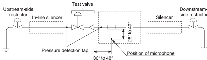
Fig. 1 Laboratory test unit by ISA-RP59.1
